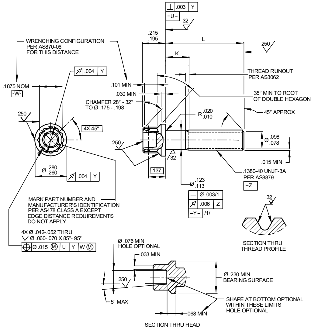
FIGURE 1 - SCREW
